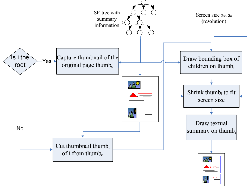
Fig. 7. Textually-enhanced thumbnail generation process for an internal node in the SP-tree.
