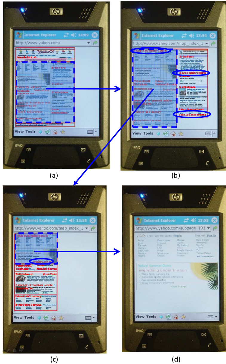
Fig. 2. Transformed pages of the original Yahoo! home page. After the user pen-taps a block in a sub-page, which is indicated by the shaded box, the corresponding sub-page of the block, which is pointed by the arrowed line, is presented to the user. The circled portions are the additional summaries that appear at the current sub-page, but not at the upper-level pages.
