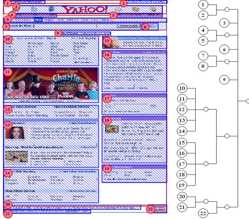
Fig. 4. The Yahoo! home page and its SP-tree, F = 8 , H = 3 , s_w = 450 , s_h = 300 .
