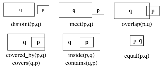
Fig. 1 Topological relations
