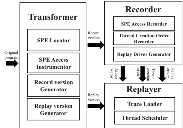
Figure 3: The overview of LEAP infrastructure
