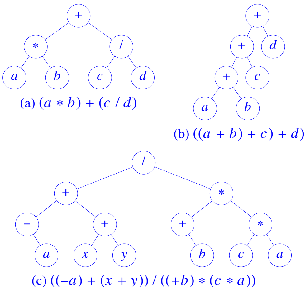
Figure 8.5 Expression trees
