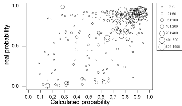
Figure 2: Final dispersion of points clustered by size
