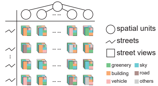
Fig. 4. Data model: street views with six-dimensional features of greenery , sky , building , road , vehicle and others , are organized in an otree structure and a street lookup table.
