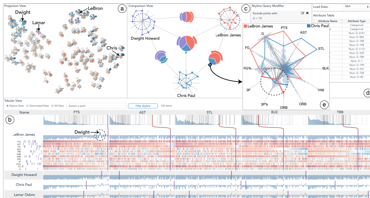
Figure 1. Analyzing the skyline of NBA statistics using SkyLens: (a) a Projection View showing an overview of clusters and outliers; (b) a Tabular View depicting the attributes of four skyline players and reveals the factors making a player in skyline; (c) a Comparison View examining the differences between skyline players from the attribute and domination perspectives; (d) a Control Panel for refining skyline queries; (e) a pop-up window showing a detailed comparison between LeBron James and Chris Paul.
