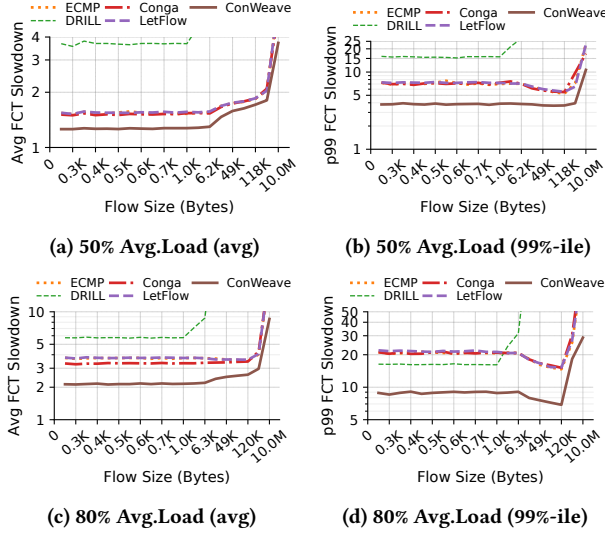
Figure 23: Avg. and 99 tail FCT slowdown for Meta Hadoop in Lossless RDMA (50% and 80% avg.load).
