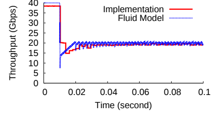
Figure 10: Fluid model closely matches implementation.
