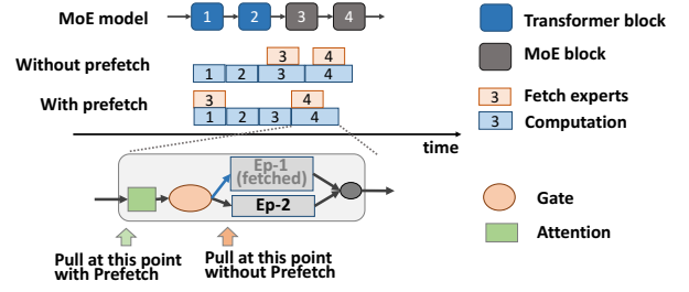
Figure 10: The concept of prefetch.
