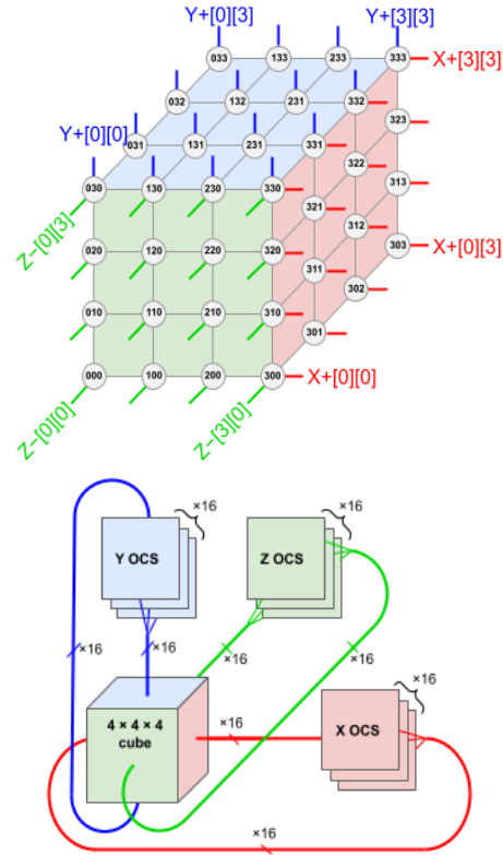
Figure 1: Connectivity of a 4 \times 4 \times 4 cube (top) to 3 OCSes (bottom). The “+” and “-” connections with the same dimension and index are connected to the same OCS; 48 of these in-out pairs each connect to a distinct OCS.
