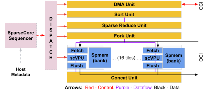
Figure 7: SparseCore (SC) Hardware Architecture.
