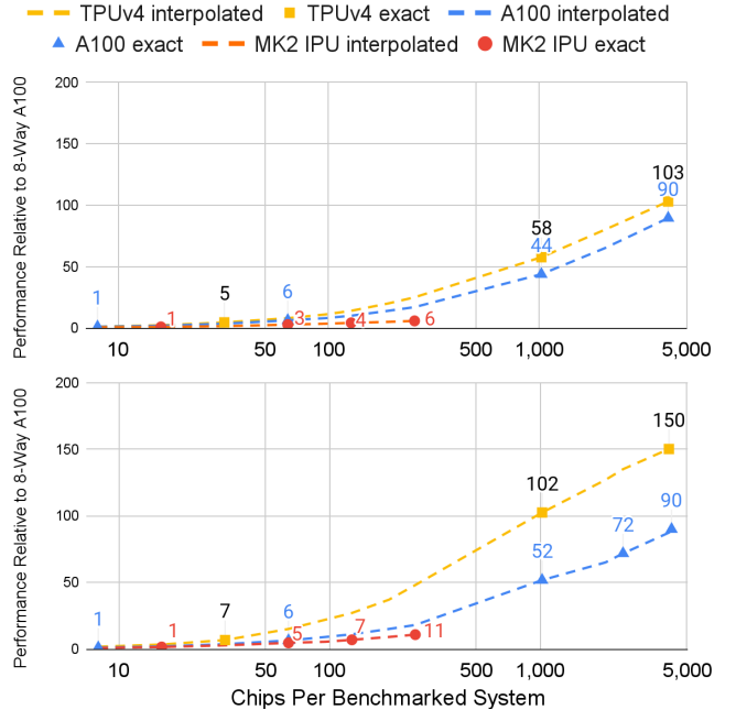
Figure 15: Reported MLPerf training 2.0 performance for BERT (top) and ResNet (bottom) [MLC22] relative to an 8-Way A100 GPU on a log-log scale. To include IPU, we only show BERT and ResNet in this figure. At the largest scale, TPU v4 is 1.15x as fast as the Nvidia A100 for BERT. At 256 chips, the maximum IPU size in MLPerf, TPU v4 is ~4.3x as fast as the MK2 IPU Bow. TPU v4 is 1.67x as fast as the Nvidia A100 for ResNet at the largest scale. At 256 chips, TPU v4 is ~4.5x as fast as the MK2 IPU Bow. The points are the reported results, and the dashed lines are interpolations for intermediate sizes systems. For TPU v4, the results below 2048 chips are from MLPerf Training 1.0; the rest of the points for all systems are from MLPerf Training 2.0.
