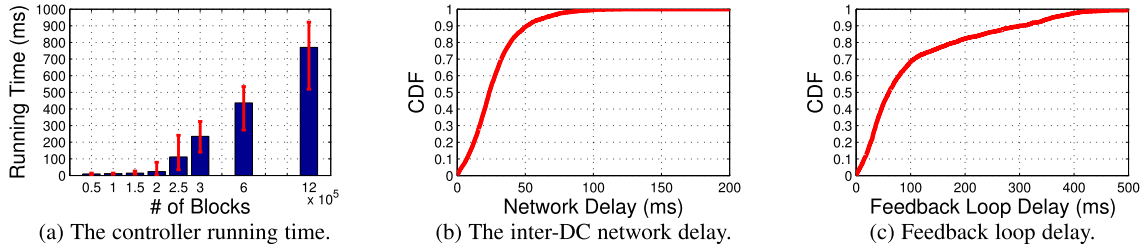
Fig. 11. [System scalability] Measurements on (a) controller running time, (b) network delay, (c) Feedback loop delay.
