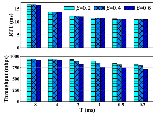
Fig. 10. RTT and throughput of inter-DC flows that bottlenecked at a WAN link. GEMINI achieves equally high throughput (944 mbps) with much lower latency ( > 7\times ) compared to TCP Cubic ( > 100 \text{ms} ).
