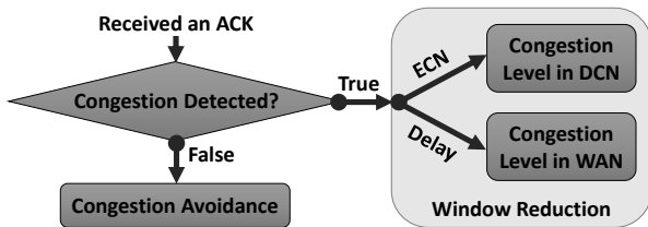
Fig. 7. GEMINI Congestion Control Process.
