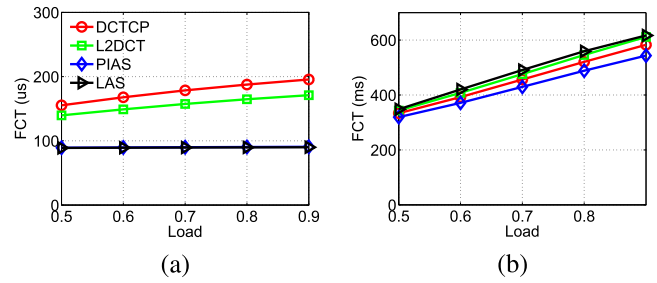
Fig. 16. Data mining workload: FCT. (a) (0,100KB]: Avg. (b) (10MB, \infty ): Avg.
