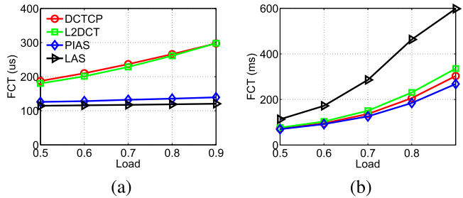
Fig. 15. Web search workload: FCT. (a) (0,100KB]: Avg. (b) (10MB,1): Avg.
