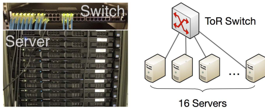
Fig. 3. Testbed Topology.
