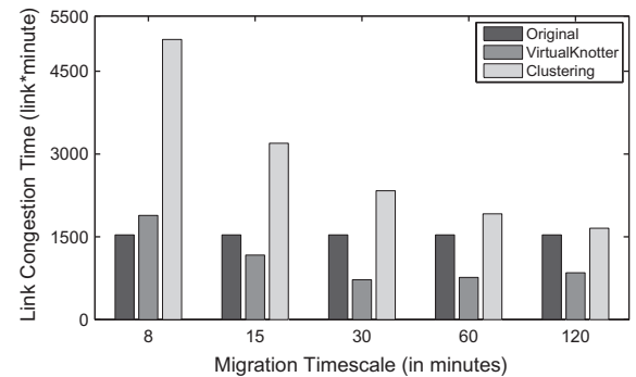
Fig. 9. Link congestion time varying replacement timescale. Congestion threshold is 0.6. All the congested time of core and aggregation links are included.
