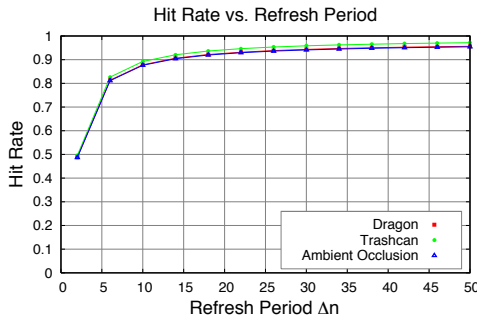
Figure 5: Hit rate as a function of refresh period for several shaders. We compare (data points) measurements to (solid lines) predictions generated by our model in Equation (4).
