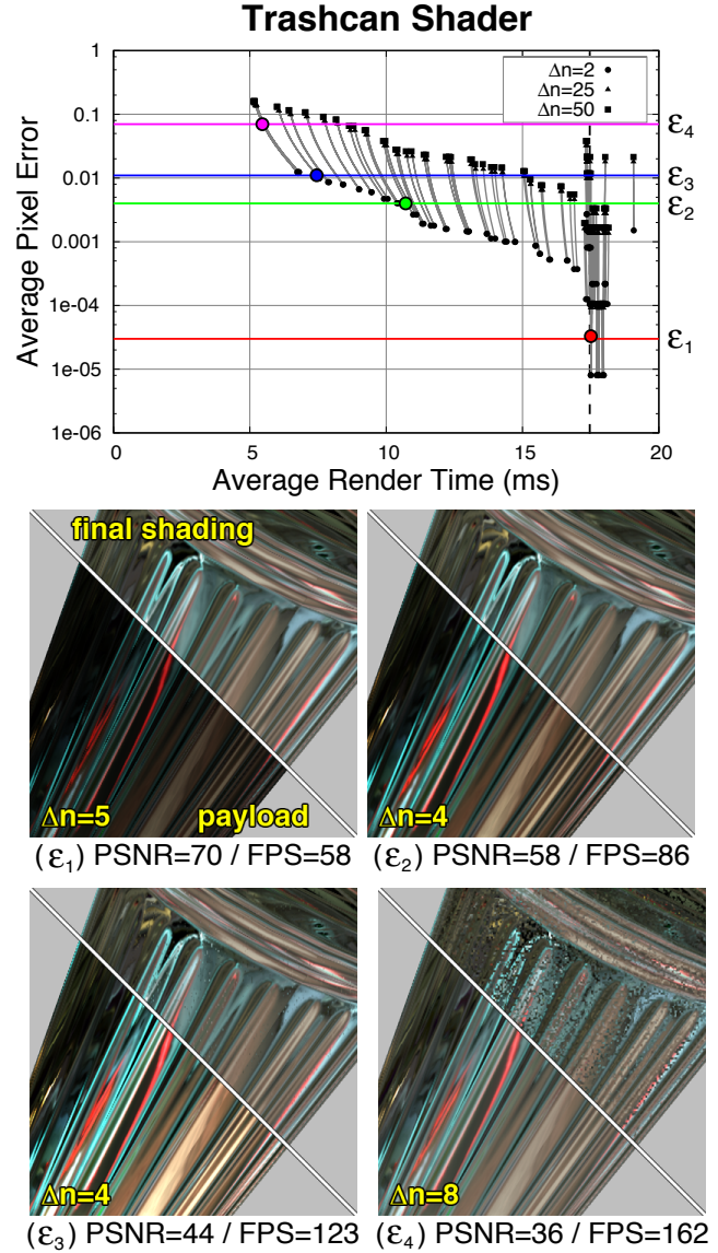
Figure 8: Error/performance paths and four selections made by our system for the Trashcan shader. The original shader runs at 59 FPS.
