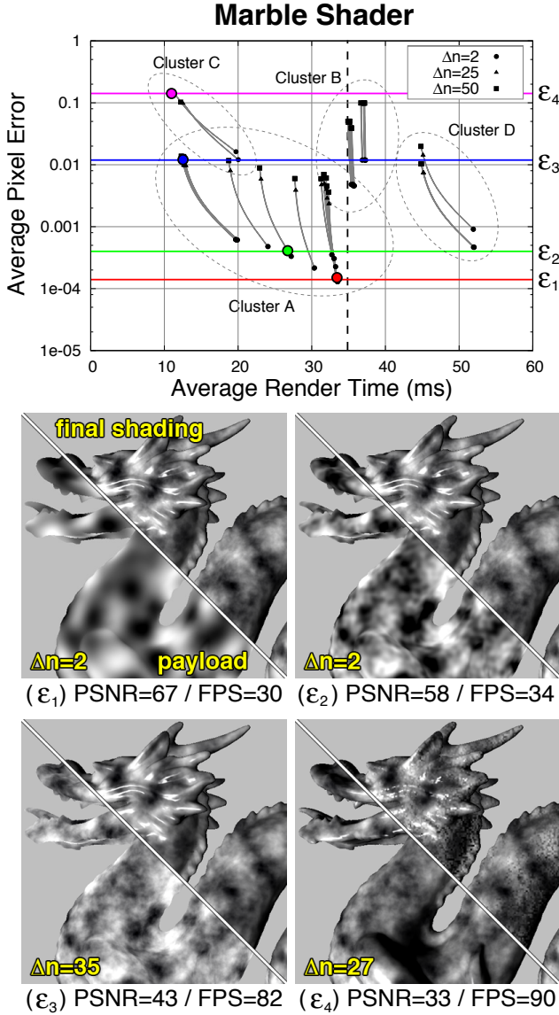
Figure 7: Error/performance paths and four selections made automatically by our system for the Marble shader. The graph at top plots the predicted average pixel error vs. render time over a range of refresh periods for each cacheable node in the AST. The images below visualize reprojection policies at four different error thresholds indicated in the graph. Each image displays the cache payload and chosen refresh period, along with the final shading and measured frame rate. The original shader runs at 29 FPS as indicated by the dashed line.
