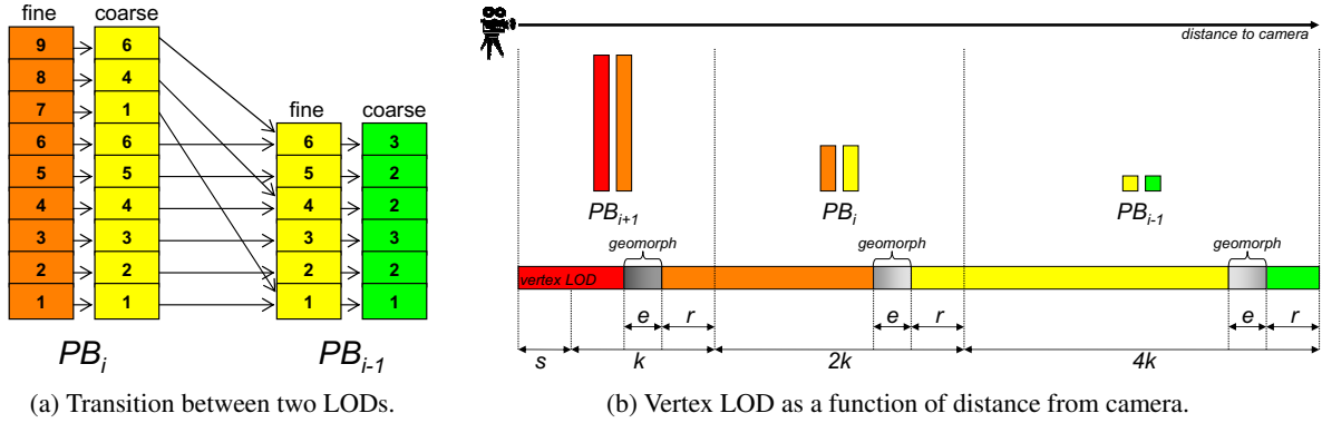
Figure 2: The geomorph depicted on the left occurs when the cluster’s bounding sphere’s center is near the transition point between rendering PB_i and PB_{i-1} . To ensure continuity, the geomorph must be performed at a distance of r away from this transition point, where r is the maximum cluster radius. This is necessary so that all vertices have finished geomorphing when the cluster switches LOD. The variables k , s , and e determine the size of the LOD bands and the geomorph region.
