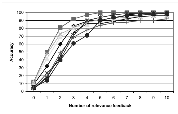
Figure 5: System performance.
