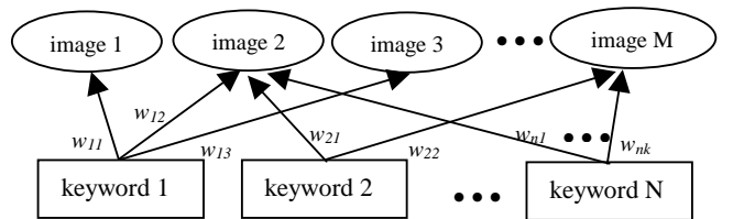
Figure 1: Semantic network
