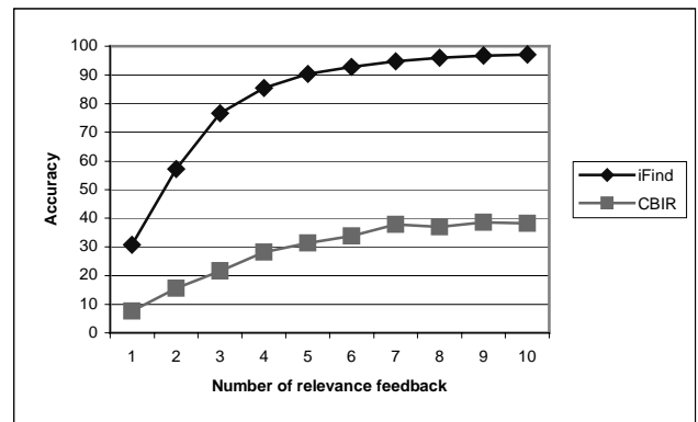
Figure 6: Performance comparison.
