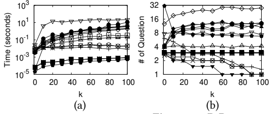
Figure 8: 2D Dataset
