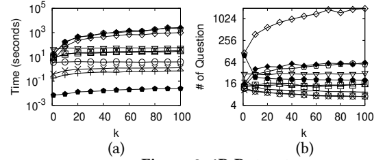
Figure 9: 4D Dataset
