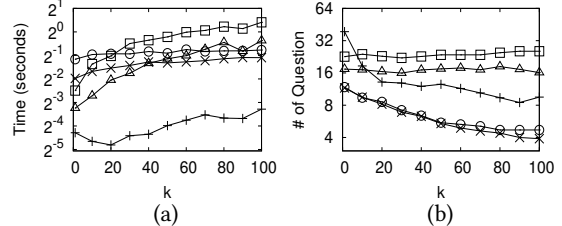
Figure 13: NBA
