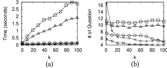
Figure 12: Weather
