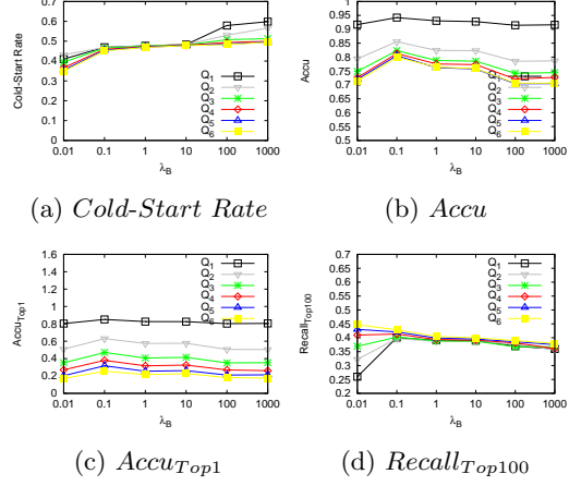
Figure 6: Impact of Parameter \lambda_B
