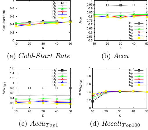
Figure 5: Impact of Parameter K
