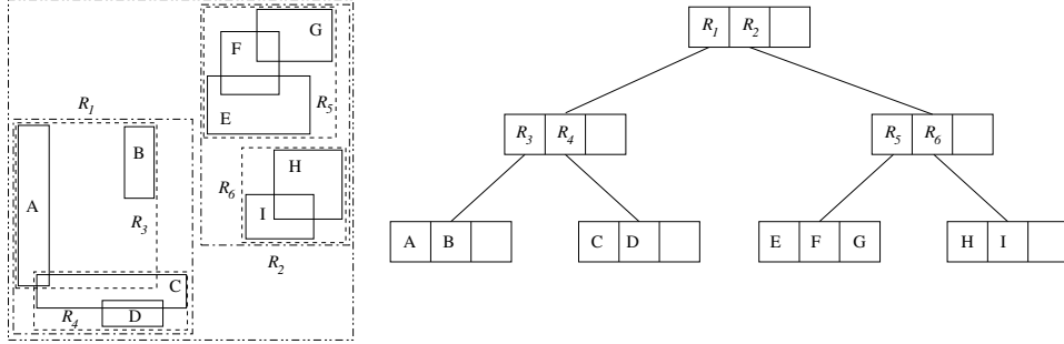
Figure 1: R-tree constructed on rectangles A, B, C, . . . , I (block size = 3).
