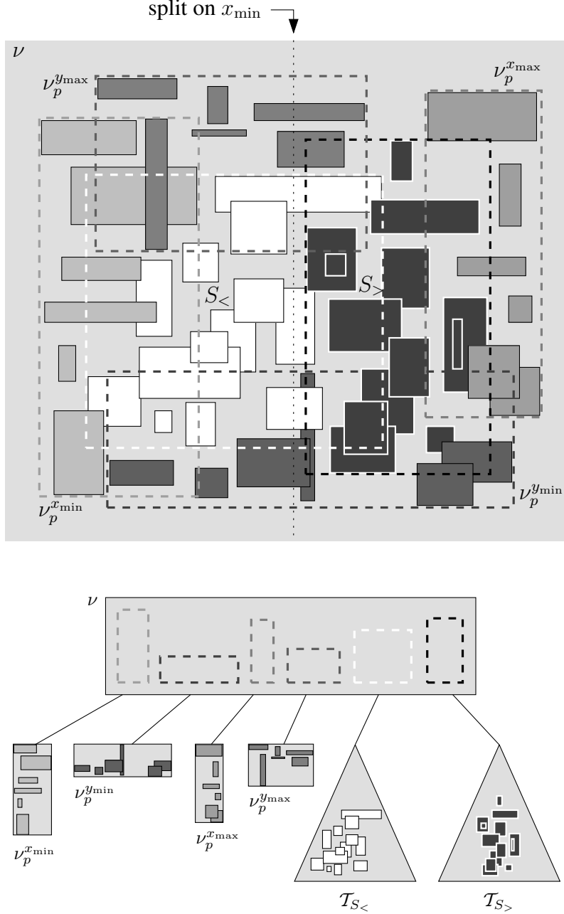
Figure 2: The construction of an internal node in a pseudo-PR-tree.
