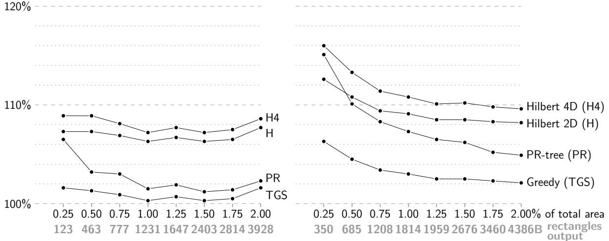
Figure 14: Query performance for queries with squares of varying size on the Western TIGER data (left) and the Eastern TIGER data (right). The performance is given as the number of blocks read divided by the output size T/B .
