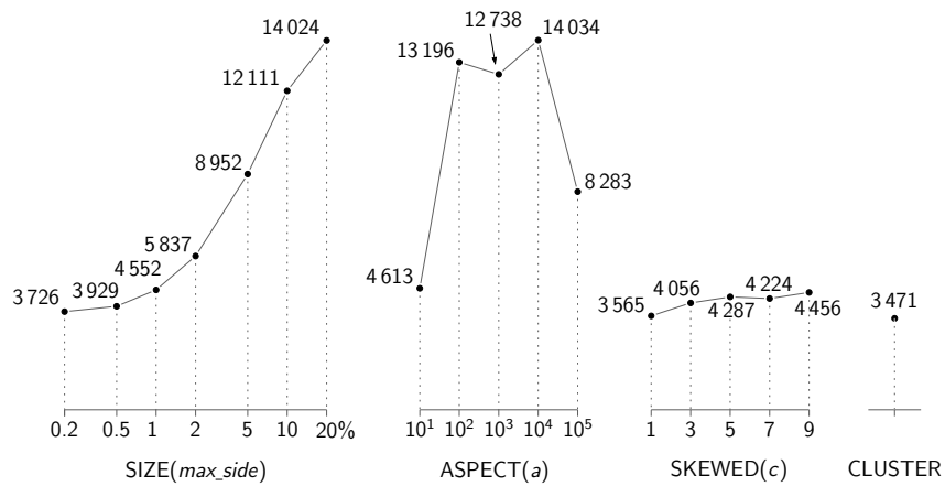
Figure 13: Bulk-loading time in seconds of Top-down Greedy Split on synthetic data sets of 10 million rectangles (SIZE and ASPECT) or points (SKEWED and CLUSTER) each.
