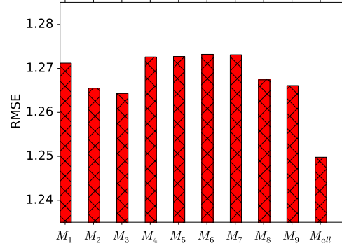
(a) Yelp.
